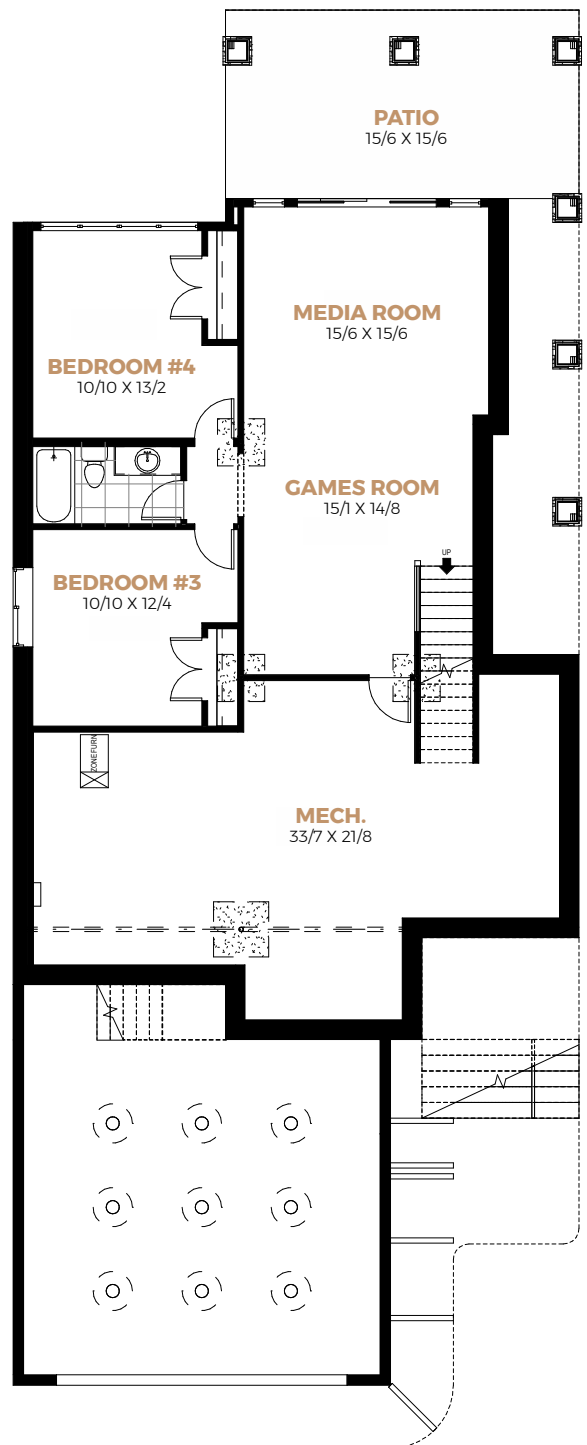
LOWER FLOOR PLAN 909 SQFT
