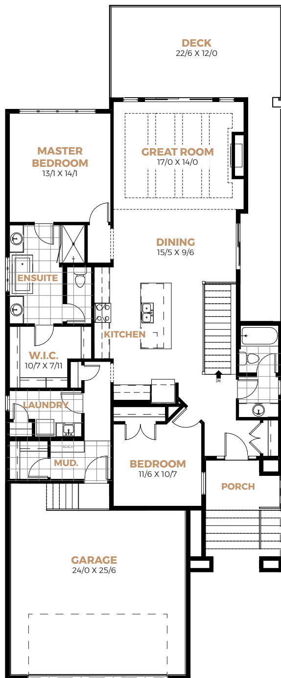
MAIN FLOOR PLAN 1,649 SQFT
