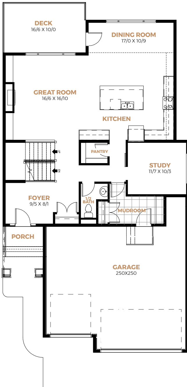
MAIN FLOOR PLAN 1,324 SQFT
